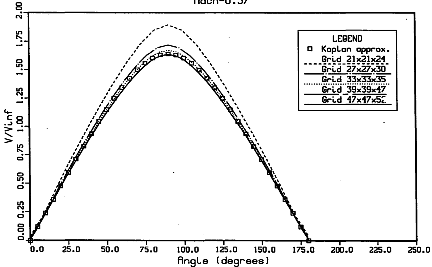
Figure 4.10: The effect of grid refinement on the Poisson solution for a sphere at M_{\infty} = 0.57 , and \alpha = 0^{\circ}
