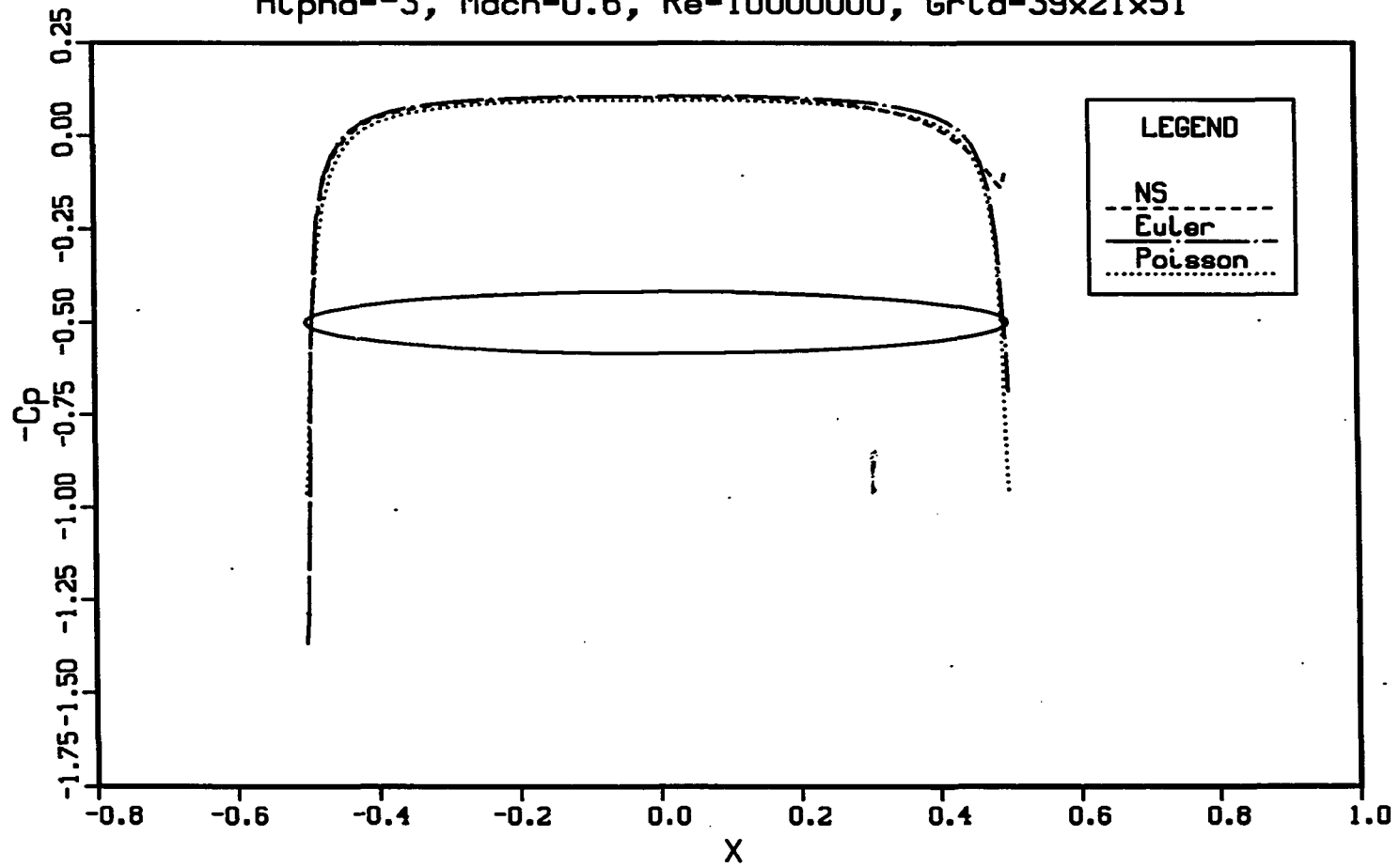
Figure 4.18: Comparison of C_p from the Poisson, Euler and Navier-Stokes solutions at the \phi = 90^\circ plane for an ellipsoid at M_\infty = 0.6 , Re = 10^7 , and \alpha = -3^\circ
