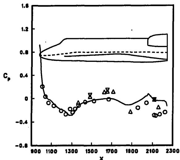
(e) M_\infty = 0.6 and \alpha = -3^\circ , Re = 4.0 \times 10^6/ft ; (computation: no elevon deflection; wind tunnel and flight: 10^\circ/9^\circ inboard/outboard elevon deflection).
