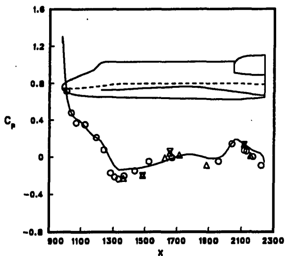
(b) M_{\infty} = 1.55 and \alpha = -6^{\circ} , Re = 3.2 \times 10^6 / ft ; (computation: no elevon deflection; wind tunnel: 10^{\circ} / -7^{\circ} elevon deflection; flight: 8^{\circ} / -5^{\circ} inboard/outboard elevon deflection, \alpha = -2^{\circ} ).
