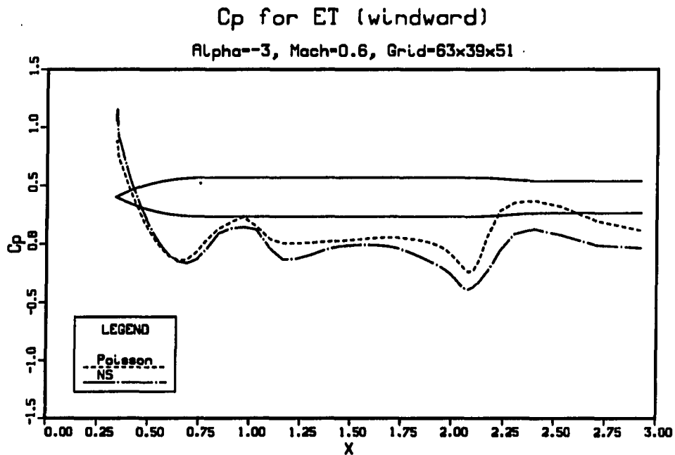
Figure 4.27: Comparison of surface pressure coefficients from the Poisson and thin-layer Navier-Stokes solutions for the ET in ISSV configuration (x in 10^3 inches)
