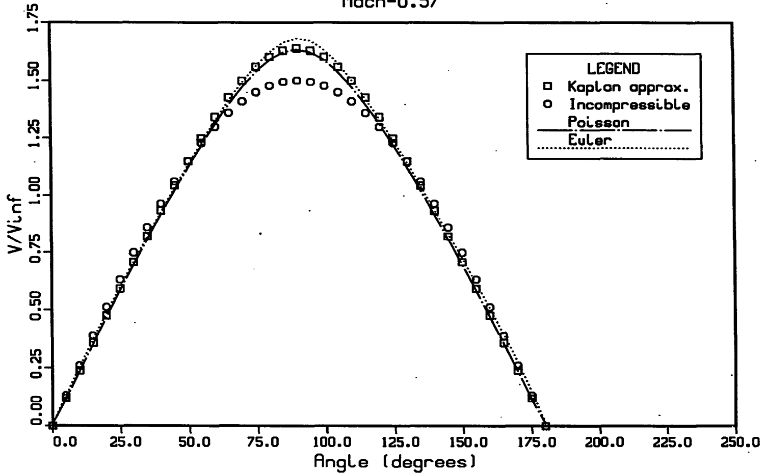
Figure 4.11: Comparison of the Poisson and Euler solutions with the analytical solution for a sphere at M_{\infty} = 0.57 , and \alpha = 0^{\circ}
