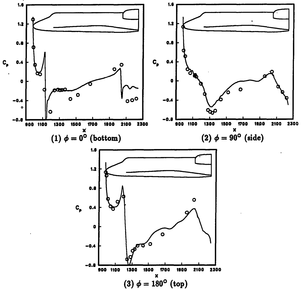
Figure 4.5: Comparison of C_p from computation (-) and wind tunnel (o) for various lines along the orbiter for M_\infty = 1.05 , \alpha = -3^\circ , and Re = 4.0 \times 10^6/ft ( x in inches)
