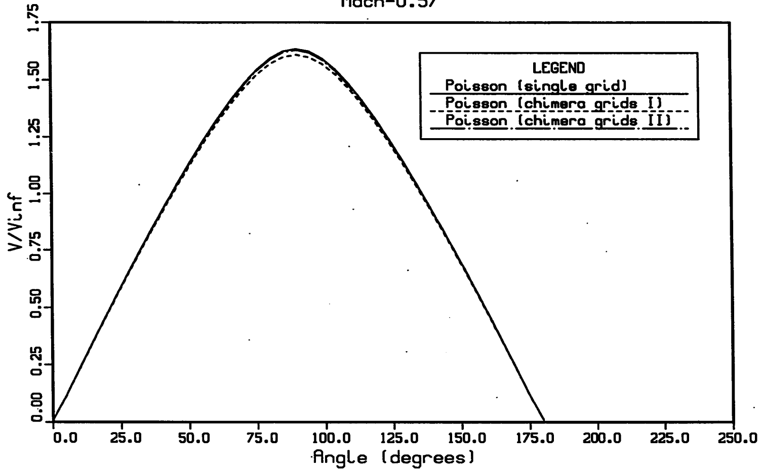
Figure 4.13: Surface velocity comparisons of the single and chimera grid solutions for a sphere at M_{\infty} = 0.57
