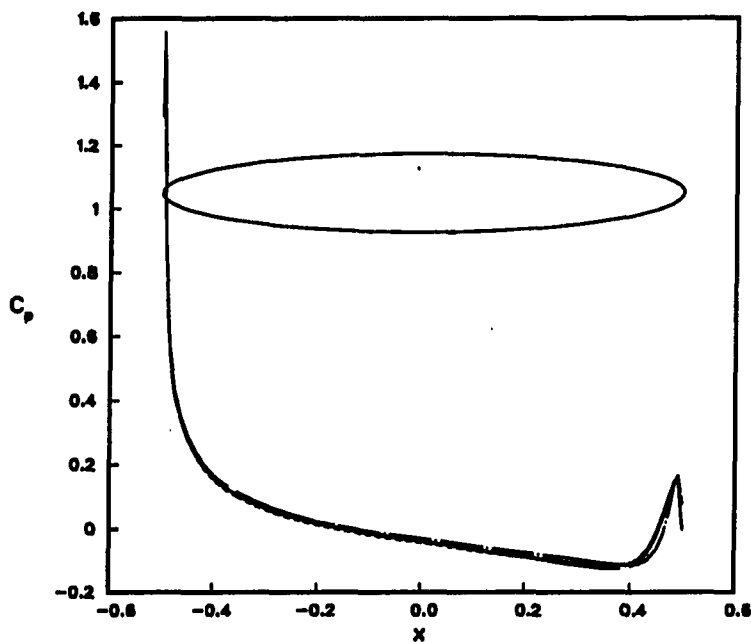
(b) Windward, combined Poisson and thin-layer Navier-Stokes solutions.
