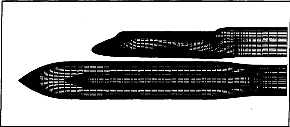
Figure 2.4: Simplified configuration and surface grid point distributions for preliminary supersonic flow calculations
