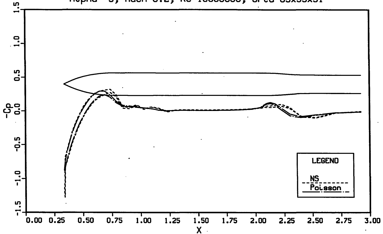
Figure 4.25: Comparison of surface pressure coefficients for the external tank, M_{\infty} = 0.2 , Re = 4.0 \times 10^6/ft , and \alpha = -3^{\circ} ( x in 10^3 inches)
