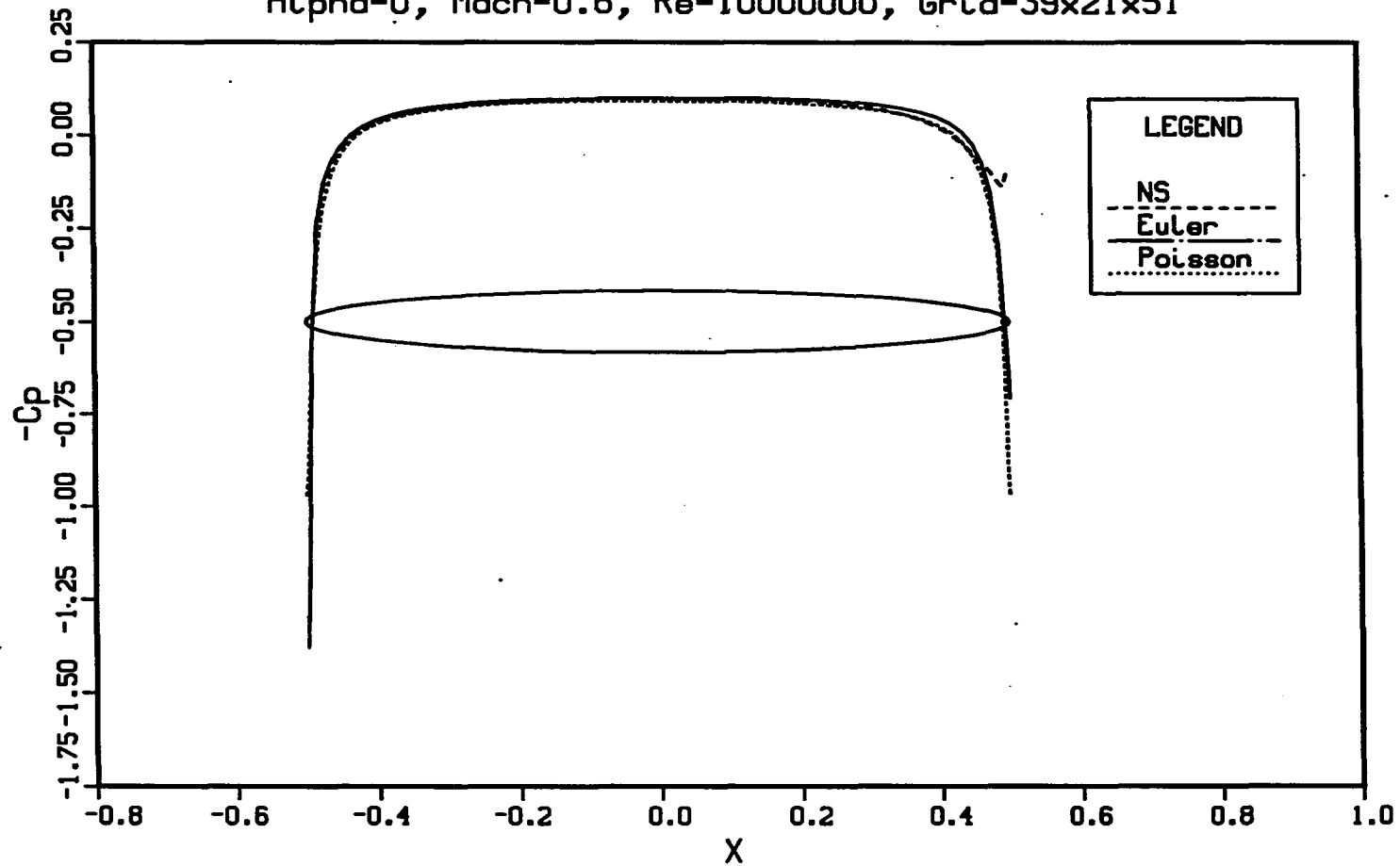
Figure 4.15: Comparison of C_p from the Poisson, Euler and Navier-Stokes solutions at the plane of symmetry for an ellipsoid at M_\infty = 0.6 , Re = 10^7 , and \alpha = 0^\circ
