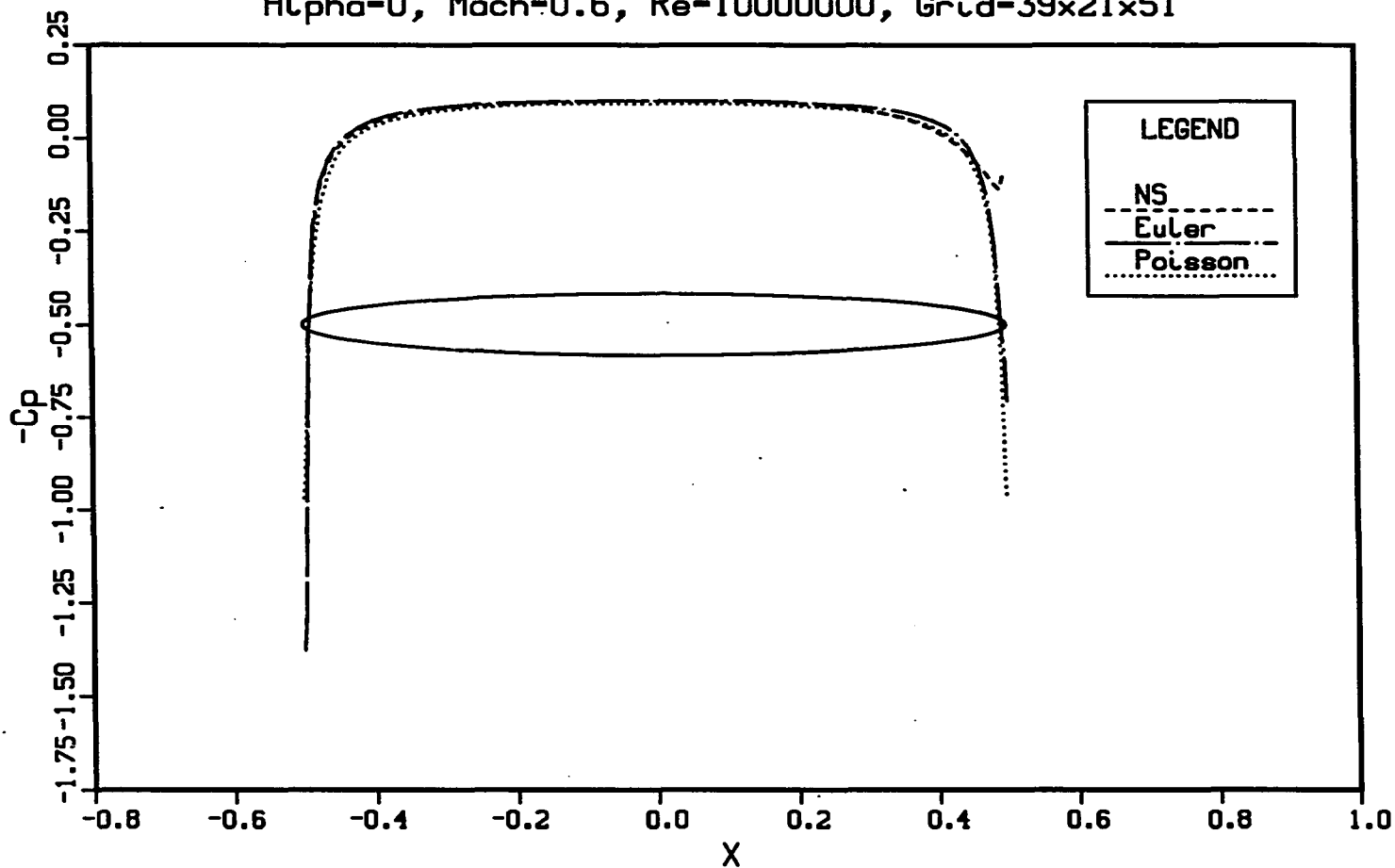
Figure 4.16: Comparison of C_p from the Poisson, Euler and Navier-Stokes solutions at the \phi = 90^\circ plane for an ellipsoid at M_\infty = 0.6 , Re = 10^7 , and \alpha = 0^\circ
