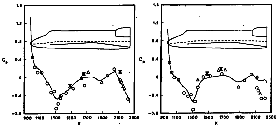
(c) M_\infty = 1.05 and \alpha = -3^\circ , Re = 4.0 \times 10^6/ft ; (all: 10^\circ/9^\circ inboard/outboard elevon deflection). (d) M_\infty = 0.9 and \alpha = -3^\circ , Re = 4.0 \times 10^6/ft ; (computation: no elevon deflection; wind tunnel and flight: 10^\circ/9^\circ inboard/outboard elevon deflection).
