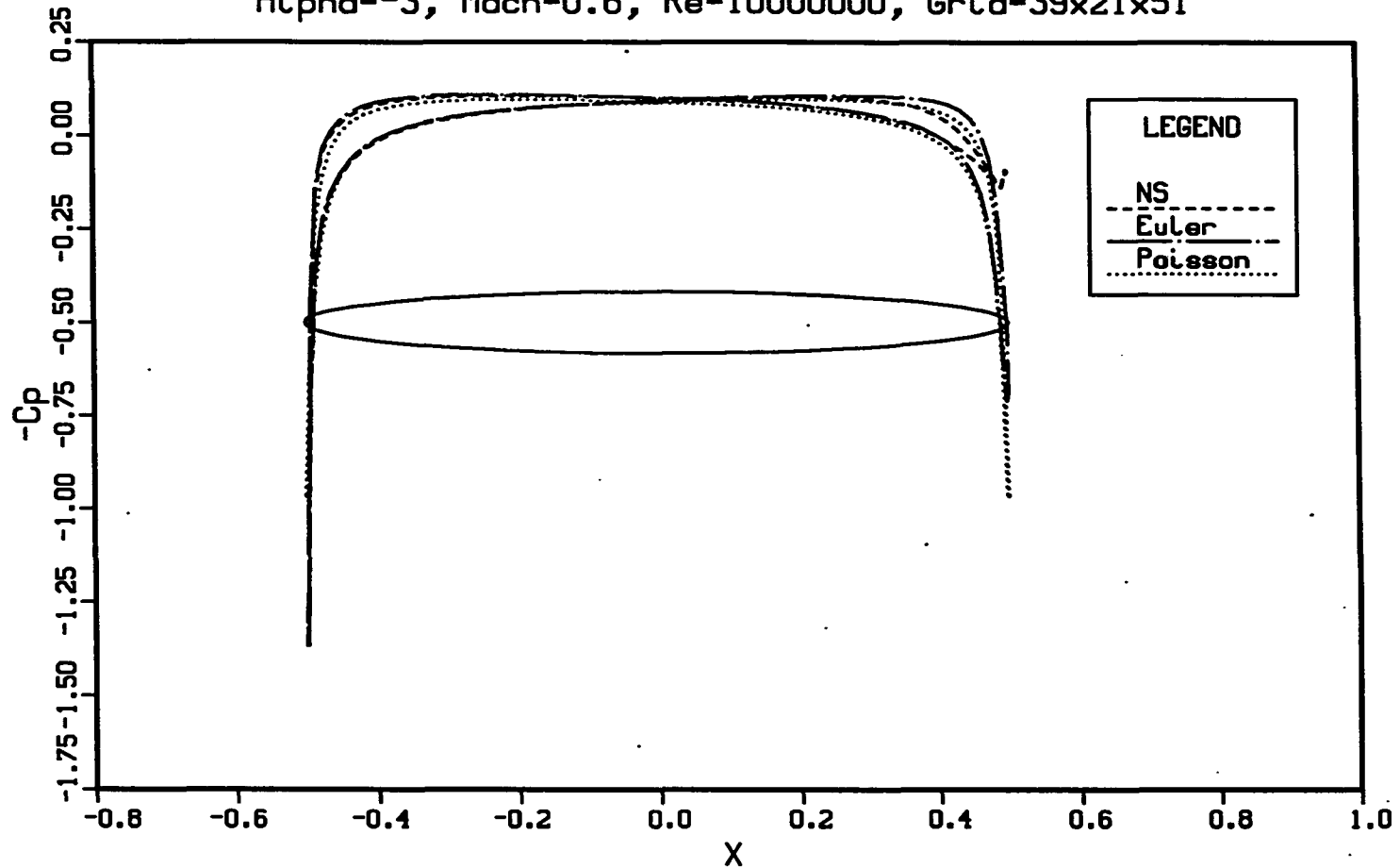
Figure 4.17: Comparison of C_p from the Poisson, Euler and Navier-Stokes solutions at the plane of symmetry for an ellipsoid at M_\infty = 0.6 , Re = 10^7 , and \alpha = -3^\circ
