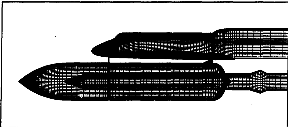
Figure 2.5: Improved configuration and surface grid point distributions
