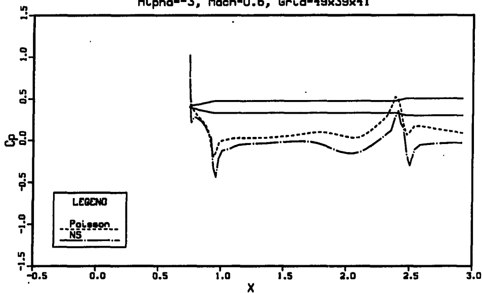
Figure 4.28: Comparison of surface pressure coefficients from the Poisson and thin-layer Navier-Stokes solutions for the SRB in ISSV configuration (x in 10^3 inches)
