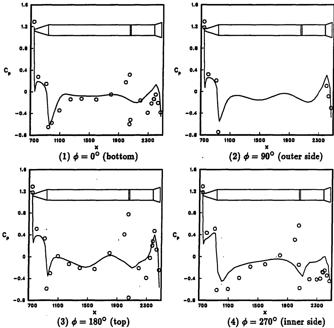
Figure 4.7: Comparison of C_p from computation (-) and wind tunnel ( \circ ) for various lines along the solid rocket booster for M_\infty = 1.05 , \alpha = -3^\circ , and Re = 4.0 \times 10^6/ft ( x in inches)
